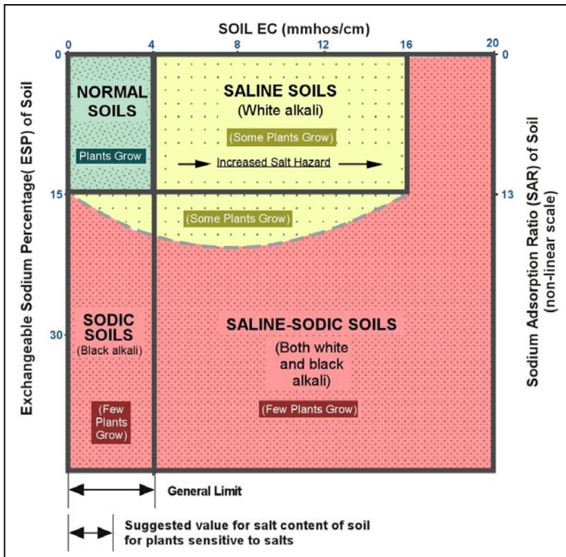
Soil Classification Based on ESP (%) (Y-Axis) and EC (mmhos/cm) (X-Axis) (API Publication 4663); adapted from Donahue et al., 1983).
