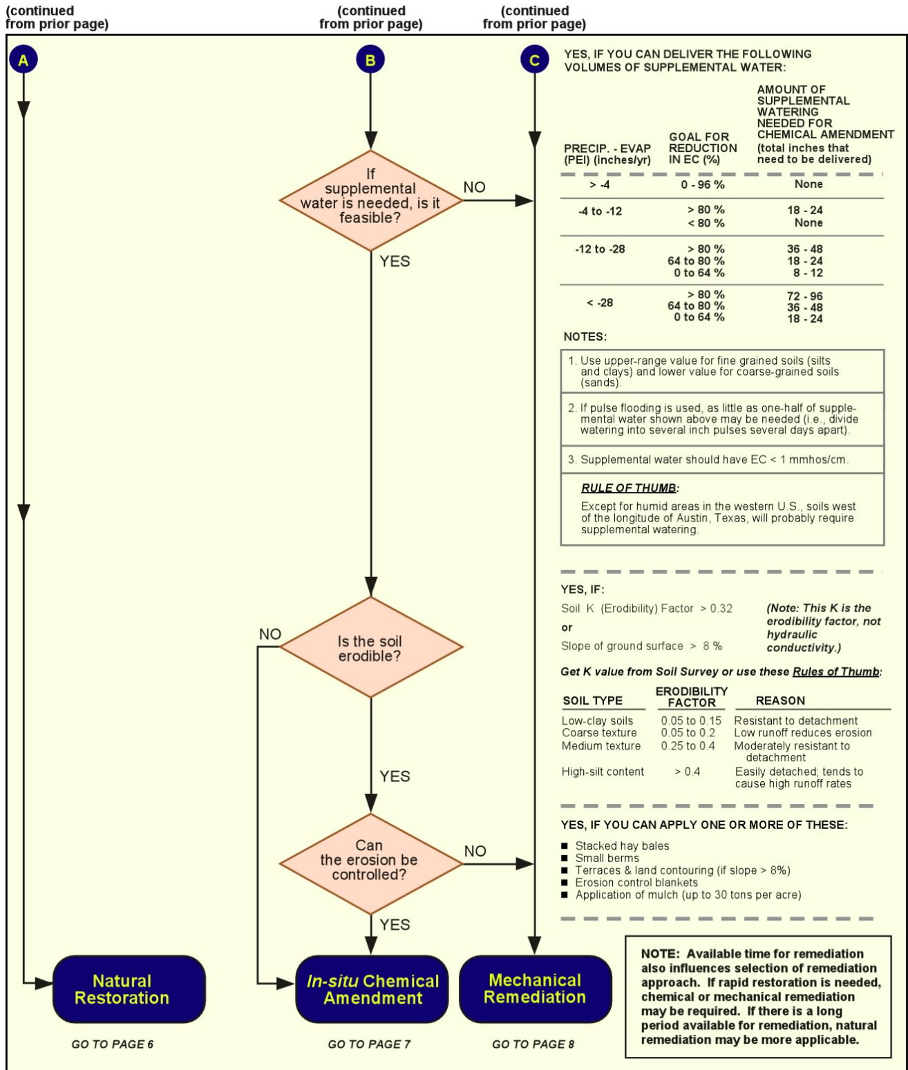
Decision Chart for Salt-Impacted Soils - Continued (Adapted from API Publication 4663)
