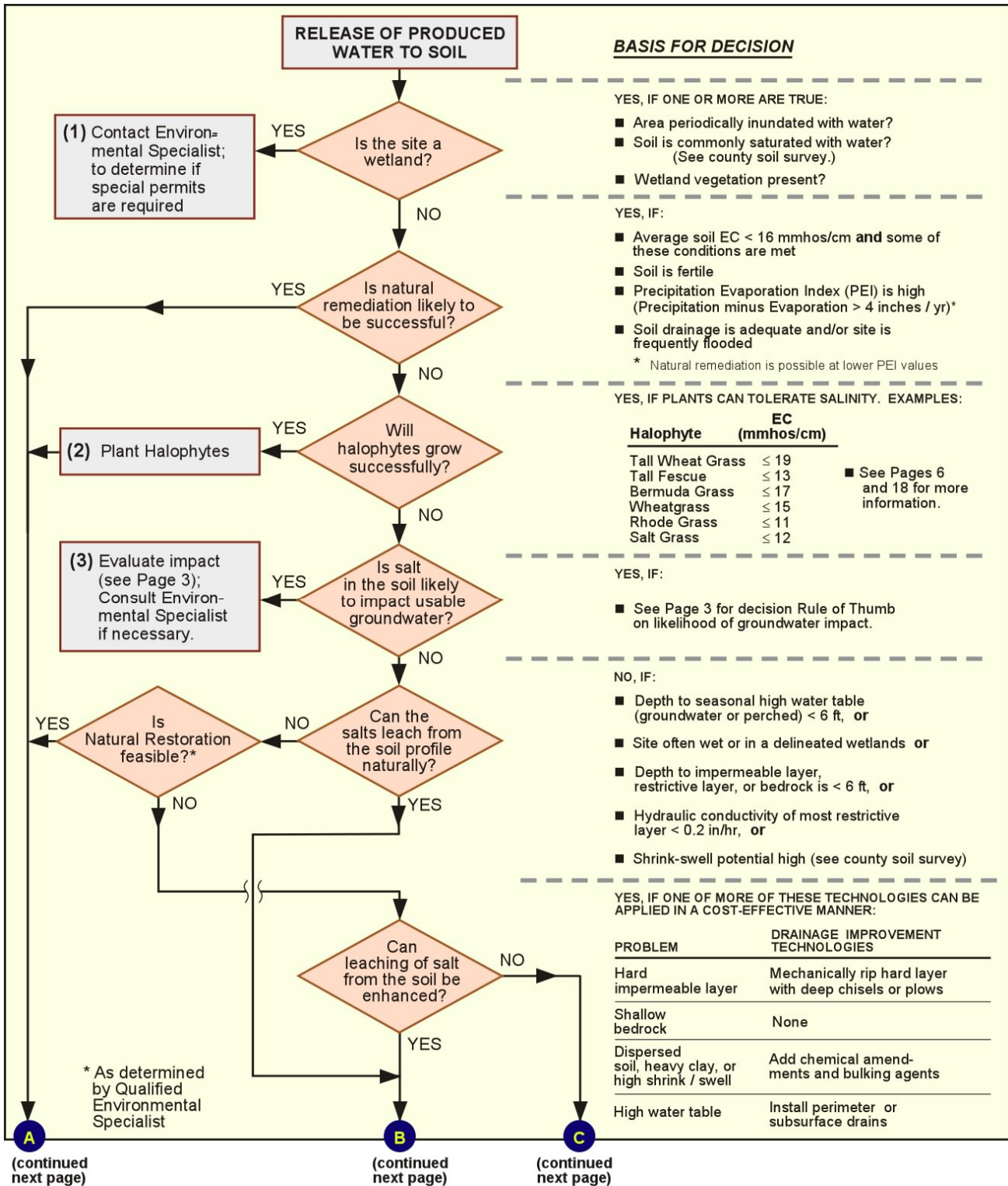
Decision Chart for Salt-Impacted Soils (Adapted from API Publication 4663)
