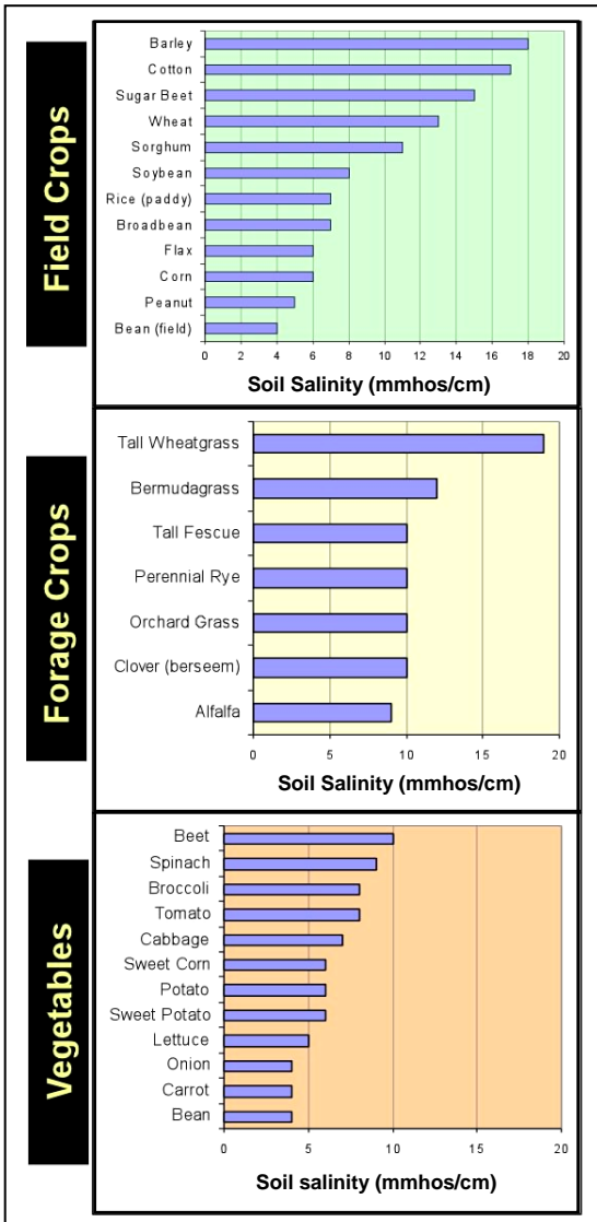
Soil Salinity Levels at Which 50% Decrease in Plant Yield is Expected. Data Compiled by Ayers and Westcot (1977).
